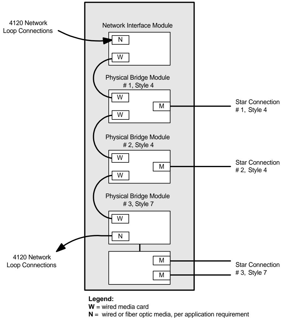
Block Diagram of a Typical Hub Node Using Physical Bridge Modules for Multiple Star Connections
