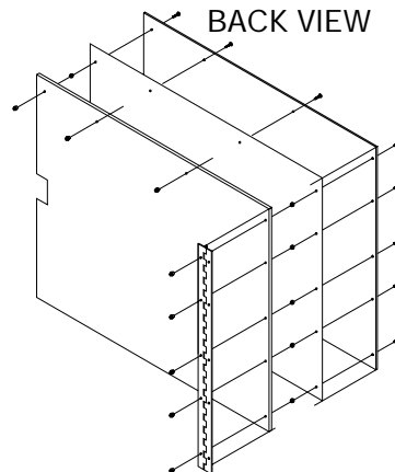
HINGE MOUNT BACK VIEW
