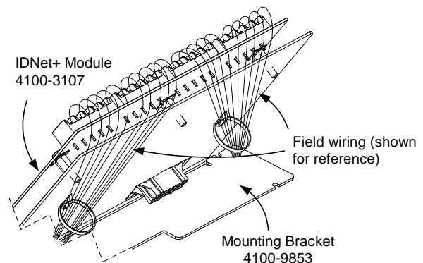
Bracket 4100-9853 with IDNet+ Module 4100-3107 Shown for Reference
