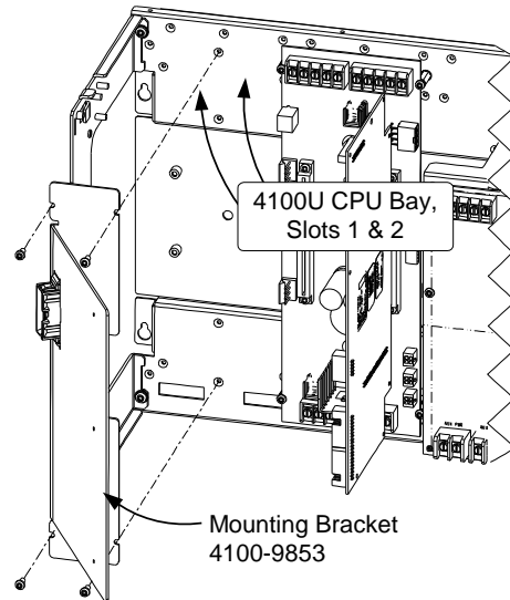
Bracket 4100-9853 Reference Drawing
