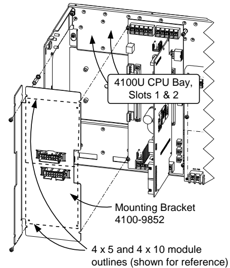
Bracket 4100-9852 Reference Drawing
