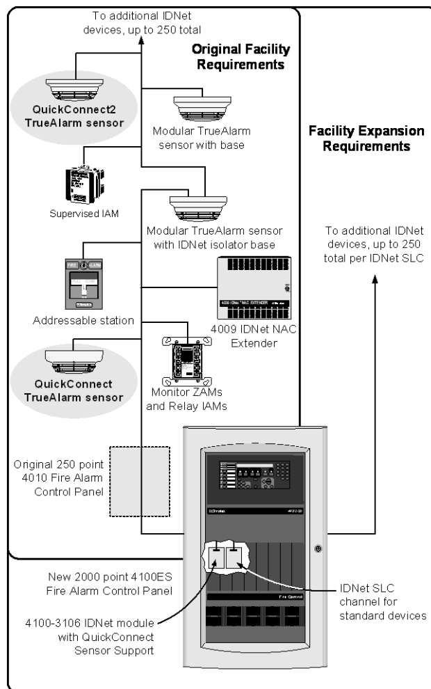
4010 System Expansion using a 4100-3106 IDNet Module
