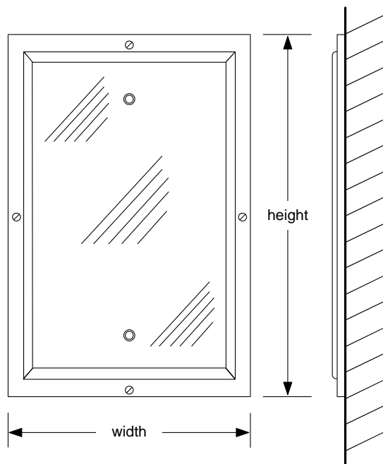
Card Holder Frame (refer to chart below for models and dimensions)
