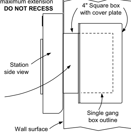
Semi-Flush Mount Side View
